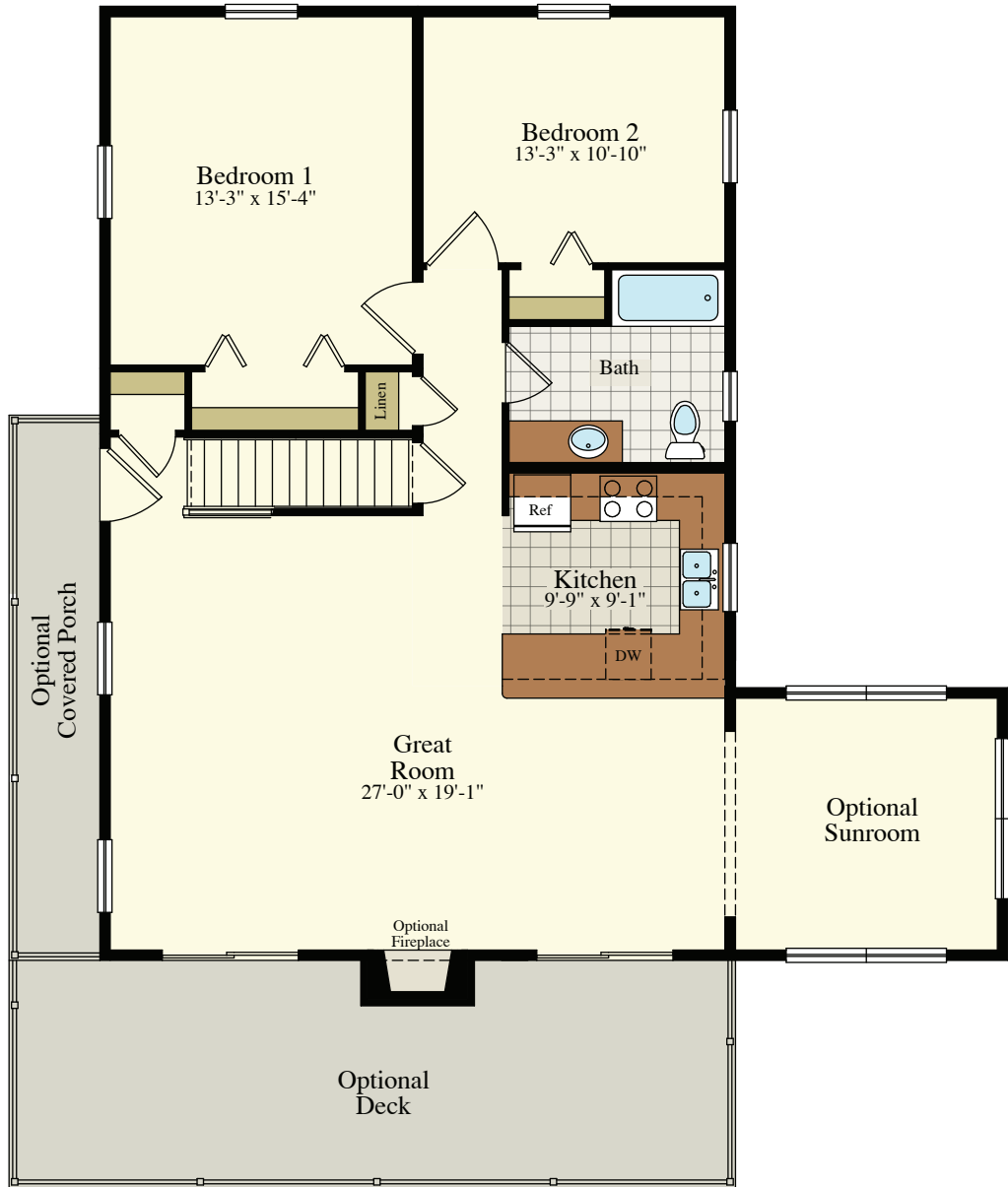
First Floor
